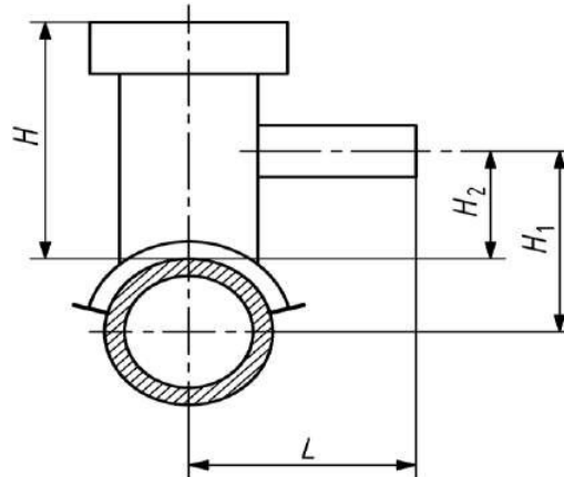
Figure 2 — Dimensions of electrofusion saddle fittings
