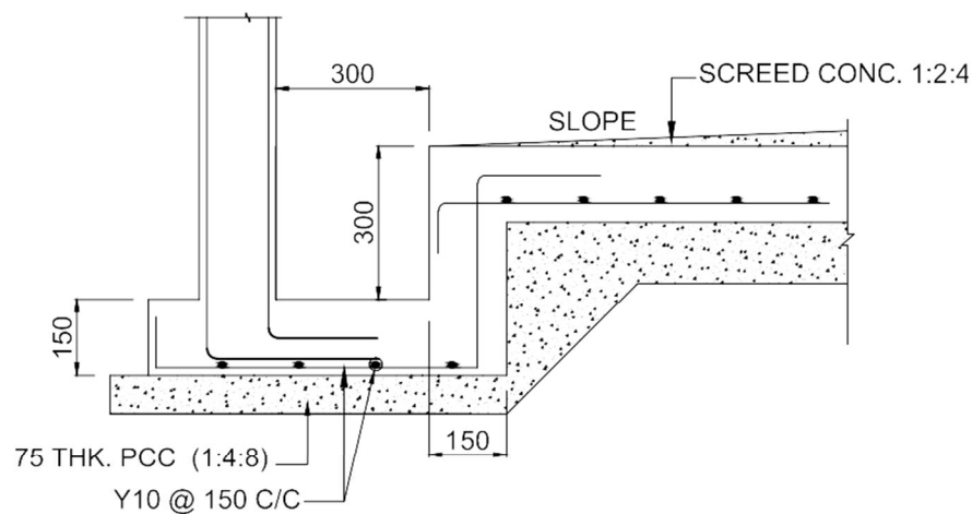
SECTION 1-1 (SCALE 1:15)
