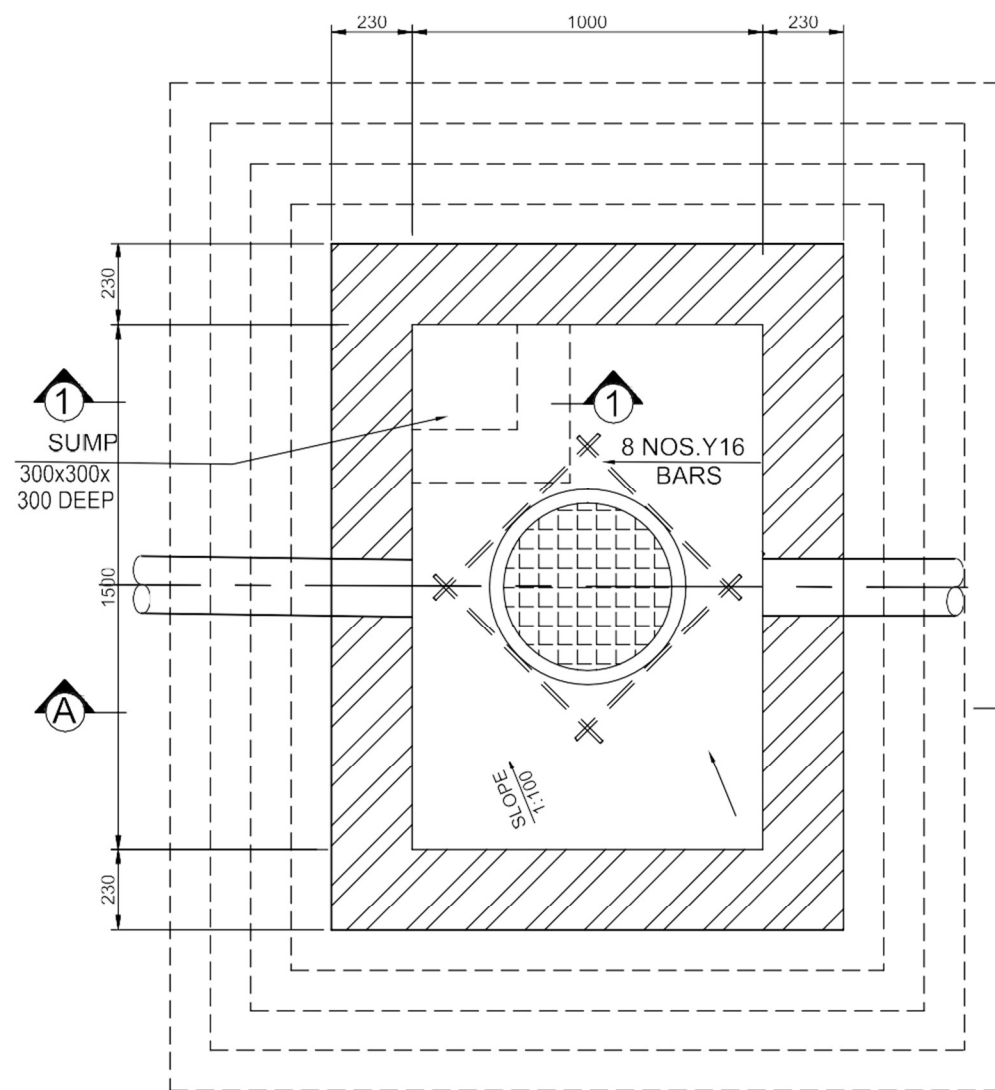
VALVE PIT PLAN (SCALE 1:20)
