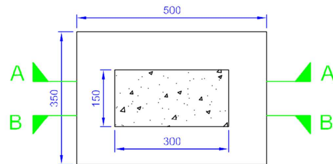
PLAIN VIEW
