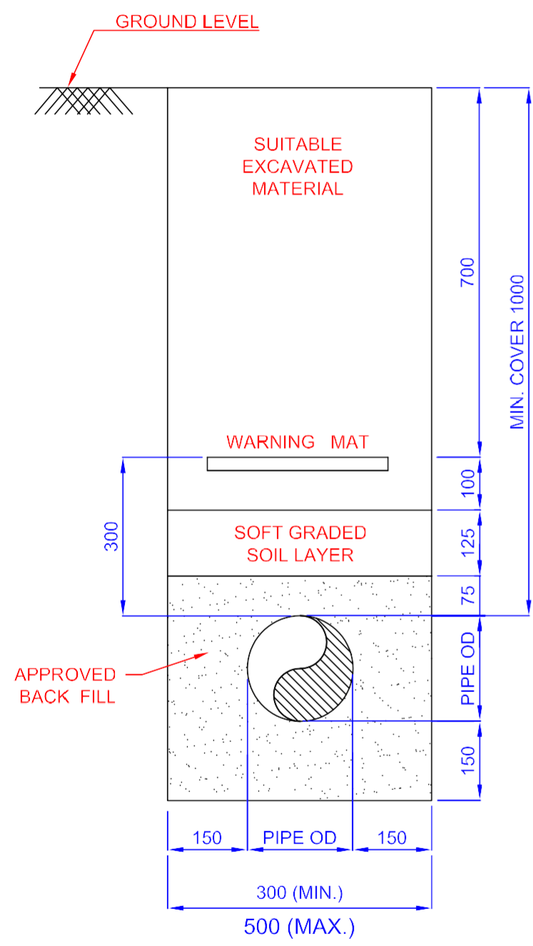
TRENCH IN ROCKY STRATA TYPICAL SECTION
