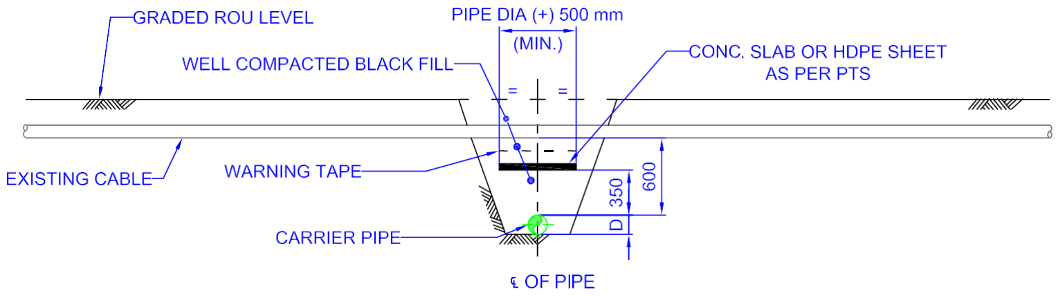
SECTION X-X
