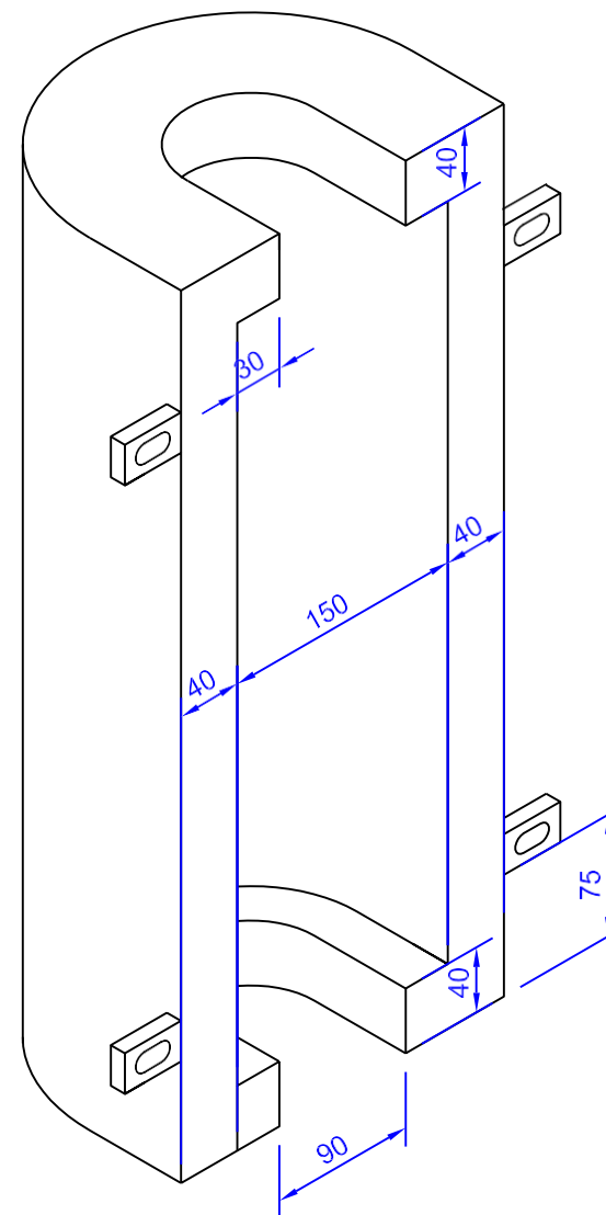
ISOMETRIC VIEW
