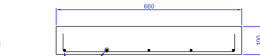
SECTION 2-2 SCALE 1:8
