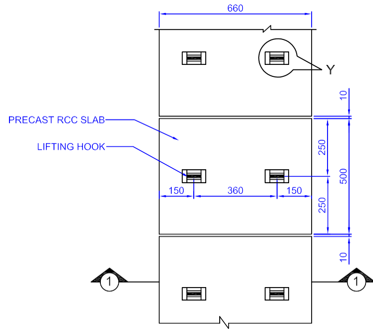
G.A PLAN OF COVER SLAB
