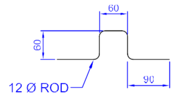
LIFTING HOOK SCALE 1:8
