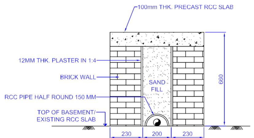
SECTION 1-1 THRU PIPE TRENCH
