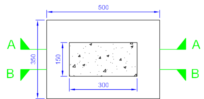
PLAIN VIEW
