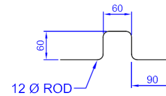
LIFTING HOOK SCALE 1:8
