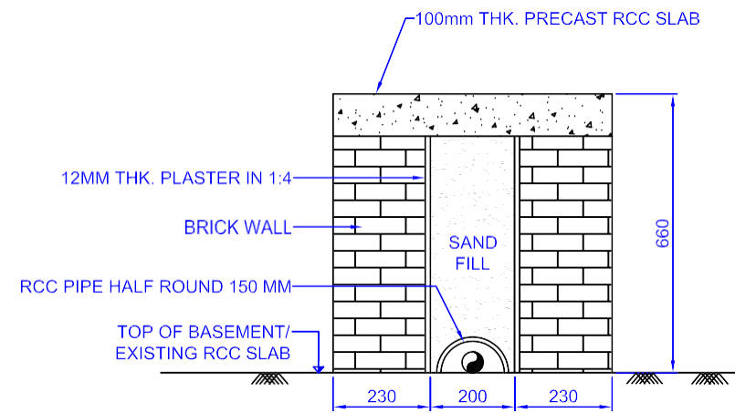
SECTION 1-1 THRU PIPE TRENCH
