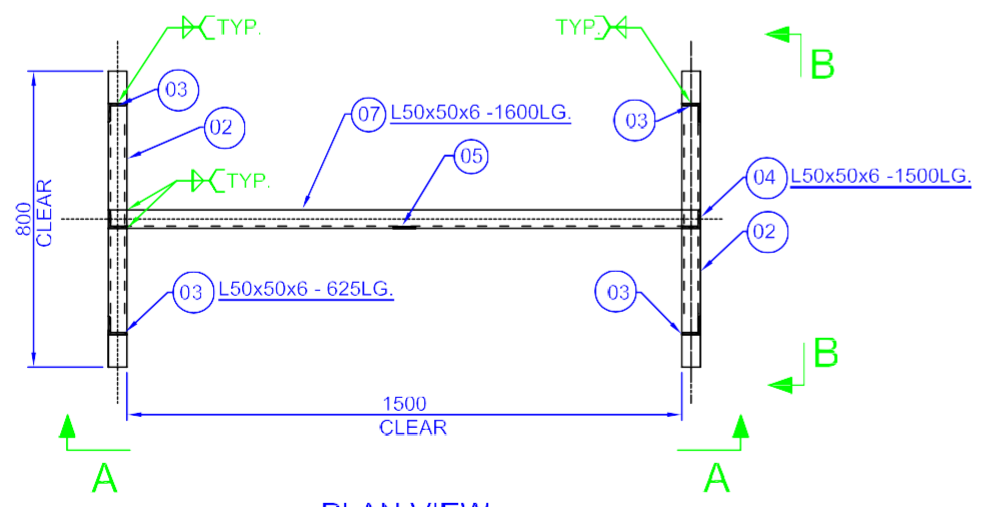
PLAN VIEW
