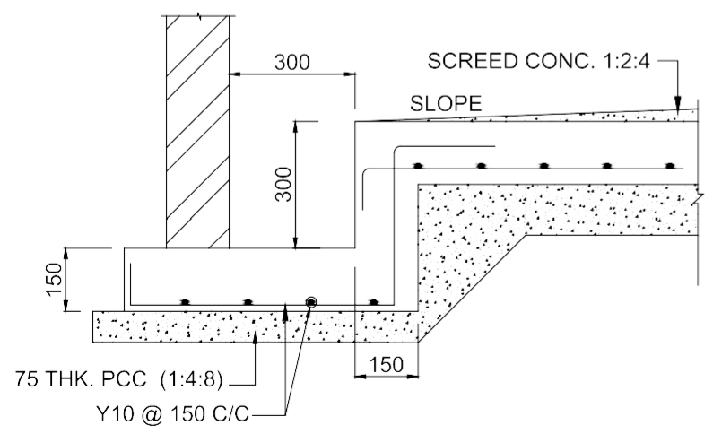
SECTION 1-1 (SCALE 1:15)
