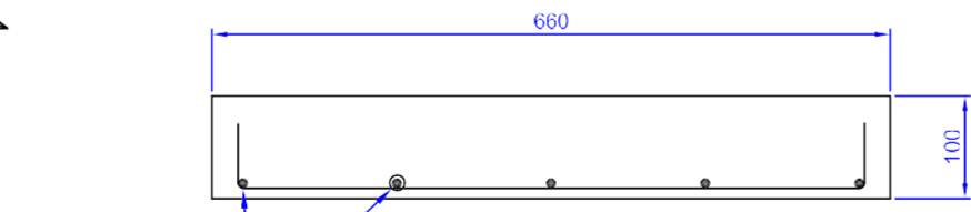
SECTION 2-2 SCALE 1:8
