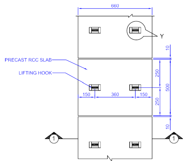
G.A PLAN OF COVER SLAB
