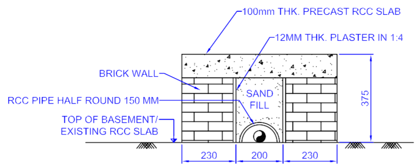
SECTION 1-1 THRU PIPE TRENCH
